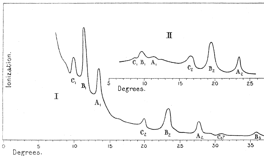
FIG. 3.—Reflection (I) from face (100) and (II) from face (111) of rock-salt. The curves show the variation of strength of reflected beam with angle of incidence.
